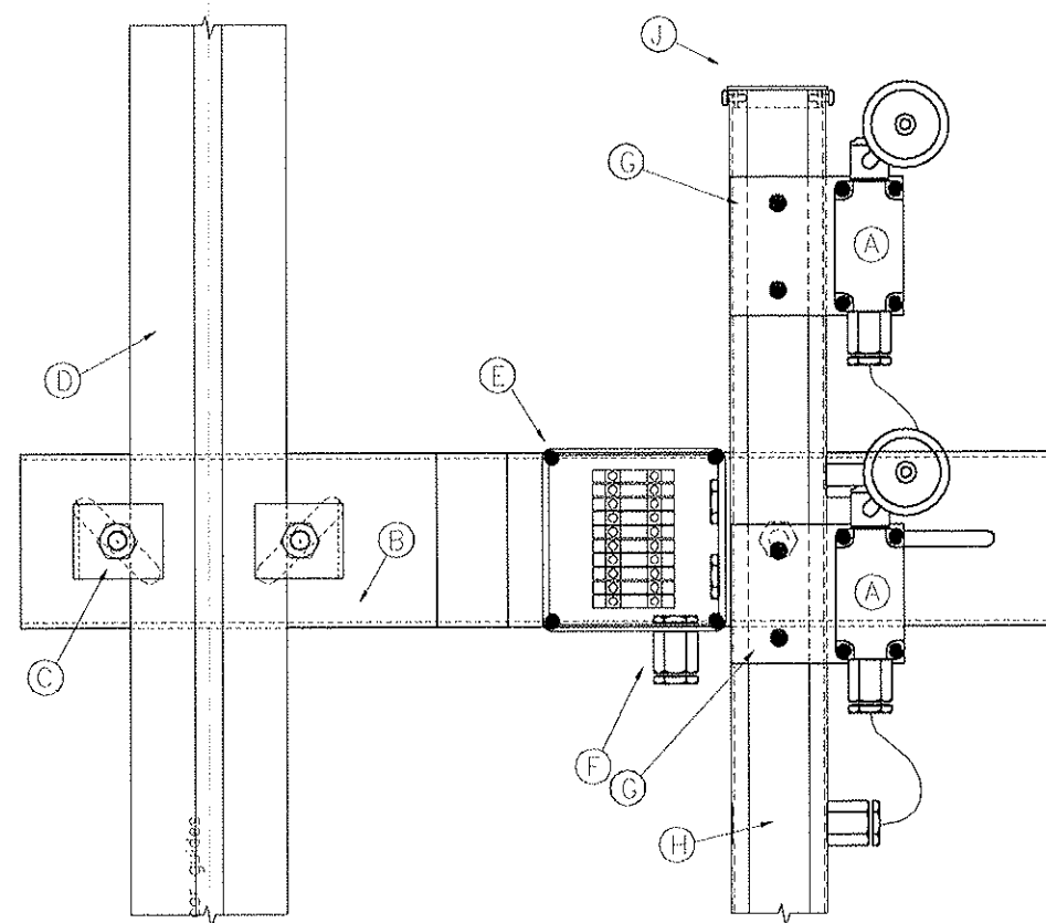
FACE VIEW of LIMIT ASSEMBLY.
